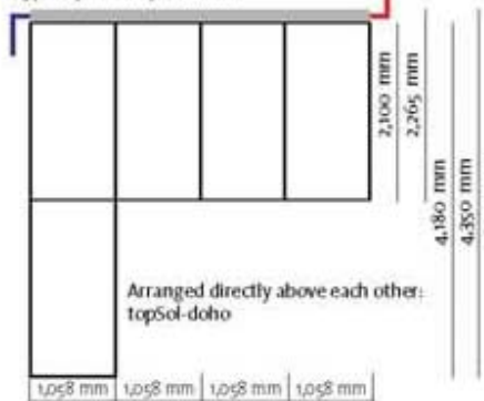
Installation dimensions type topSol + topSol-doho:
